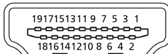
19-pin color display signal cable
