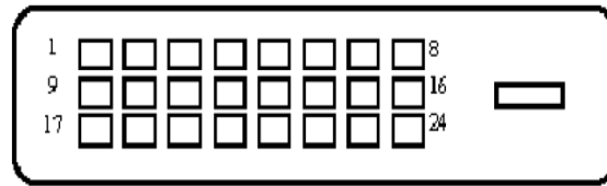
24-Pin Color Display Signal Cable
